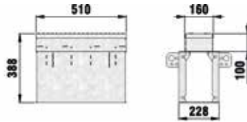
Technical drawing, inspection box
